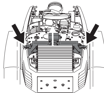
Figure 21: Dimmer module locking levers
